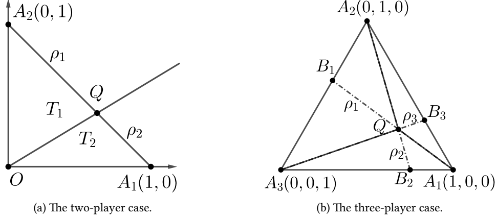
Figure 2: Simplexes for two-player and three-player cases.
