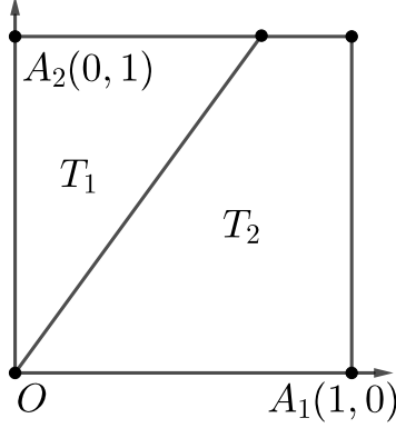
Figure 1: In the two-player case, player 1 wins if and only if the random coordinate t falls into T_1 .
